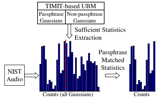
Figure 1: Passphrase-specific sufficient statistics extraction. The process of computation of the GMM counts is illustrated. Computation of the first order statistics (sums) is similar.
