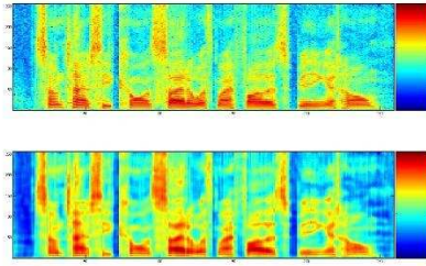
Figure 4.8. Same as Figure 4.6 but with yet another TIMIT speech utterance.
