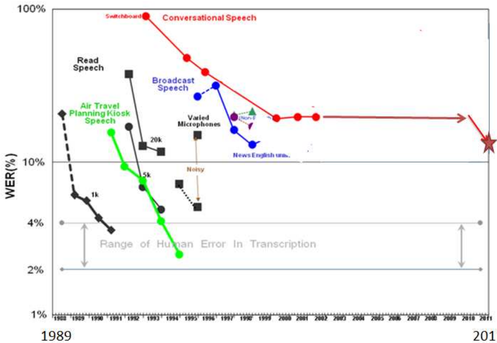
Figure 2.4. Extracting WERs of one task from Figure 2.3 and adding the significantly lower WER (marked by the star) achieved by the DNN technology approach.
