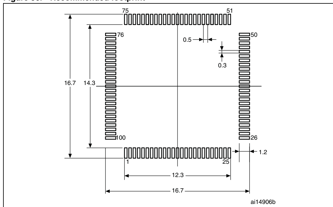
Figure 36. Recommended footprint
