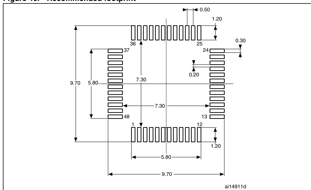
Figure 40. Recommended footprint
