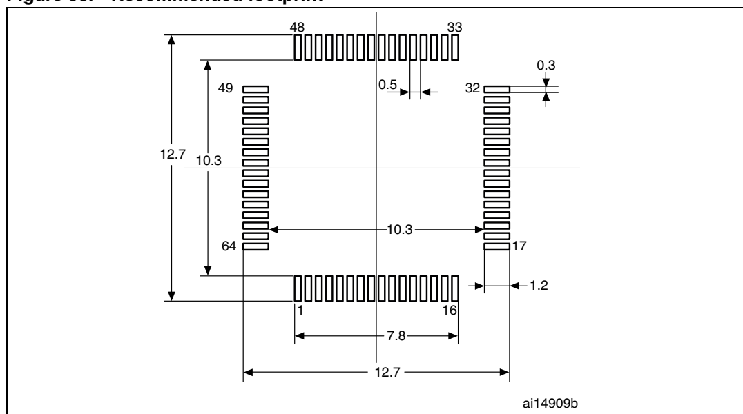
Figure 38. Recommended footprint
