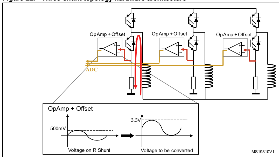
Figure 22. Three-shunt topology hardware architecture
