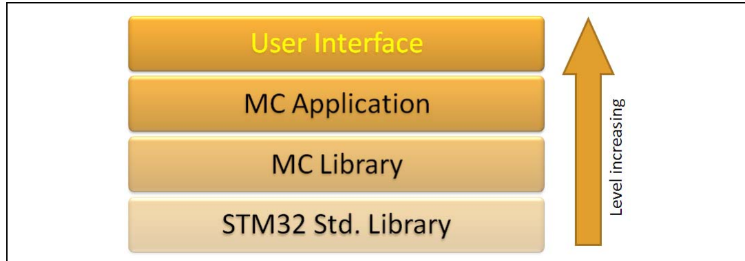
Figure 73. Software layers
