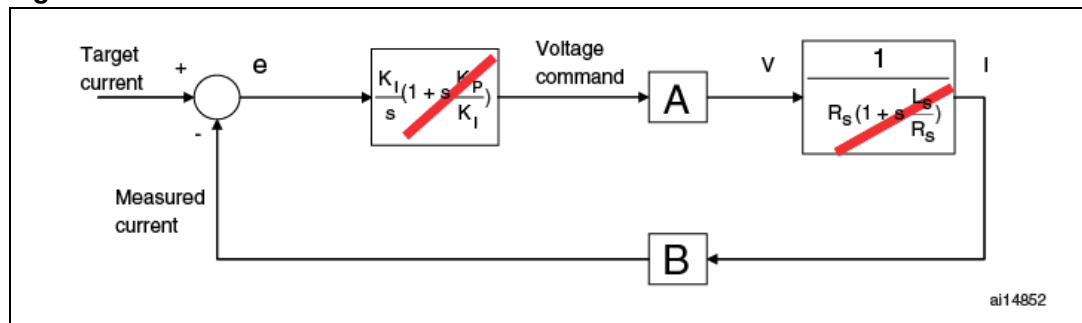
Figure 16. Pole-zero cancellation
