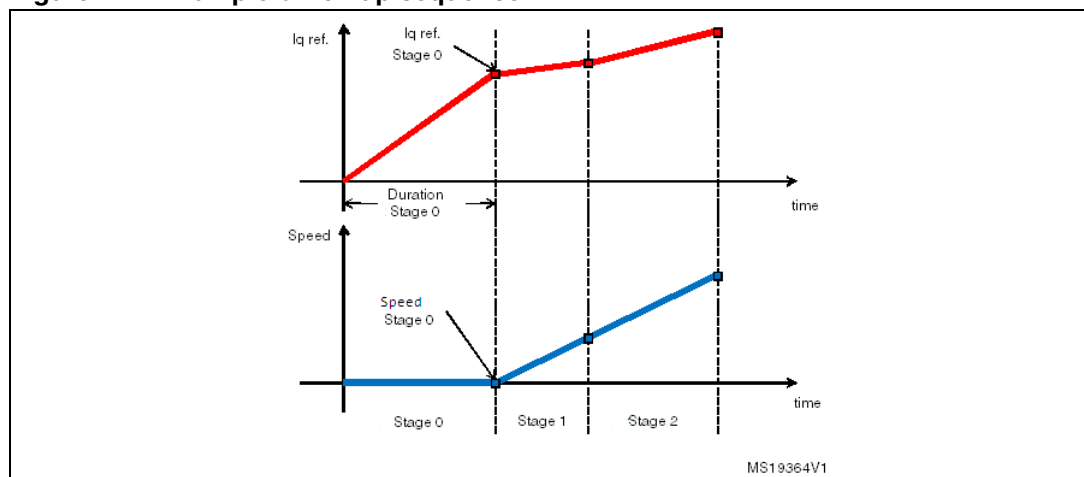
Figure 71. Example of rev-up sequence
