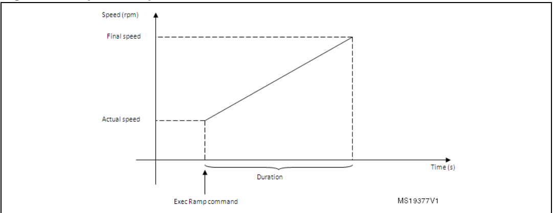
Figure 84. Speed ramp
