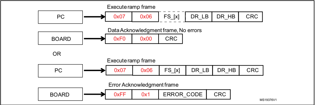
Figure 83. Execute ramp frame
