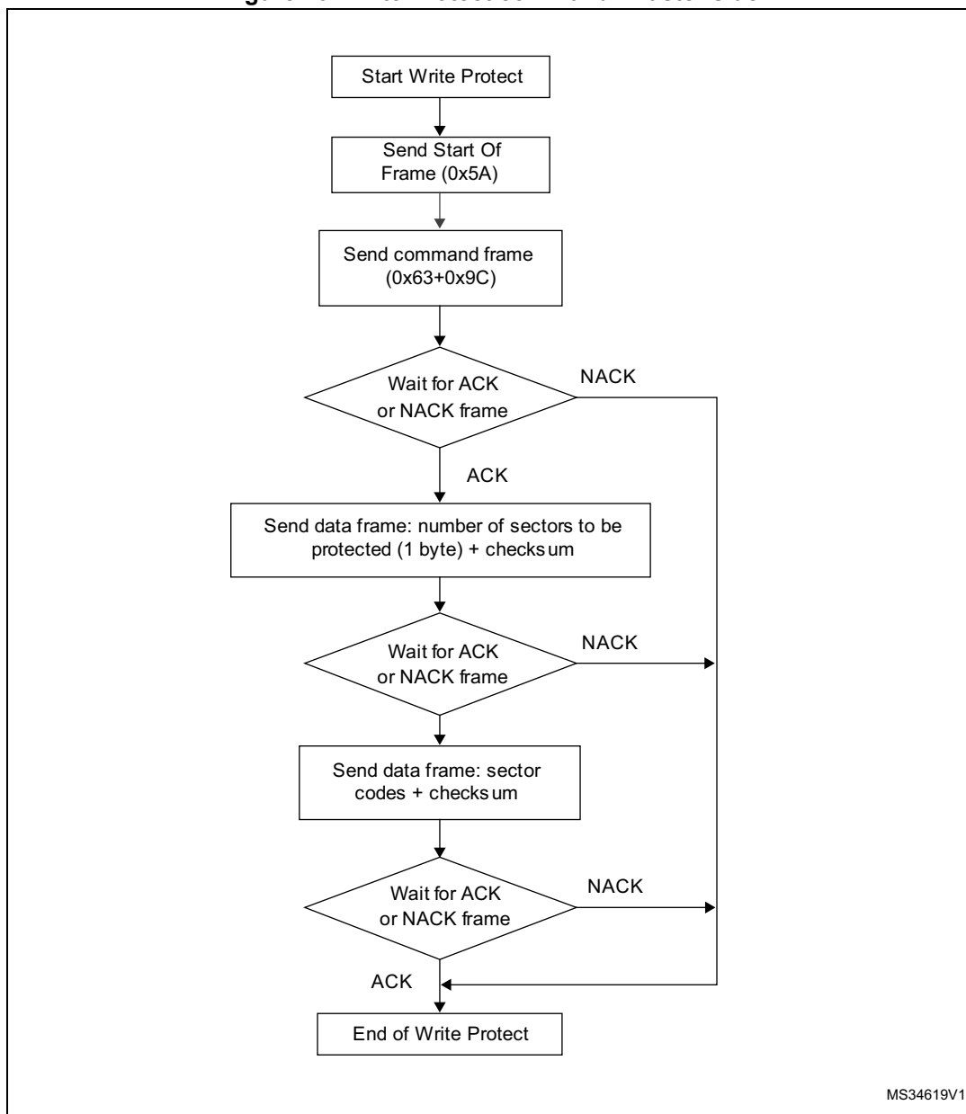
Figure 20. Write Protect command: master side
