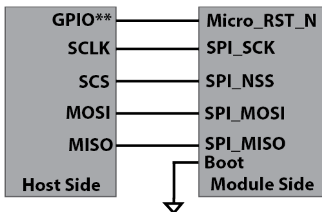
Figure 2 - SPI Host Interface Reference Diagram
