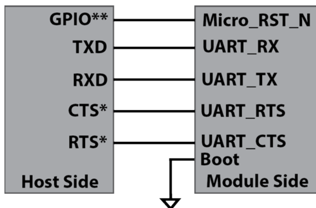
Figure 1 - UART Host Interface Reference Diagram
